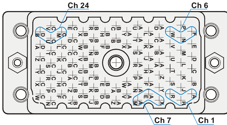
90 pole EDAC male (mating side)
