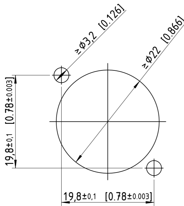
Panel cut out(Rear side)
