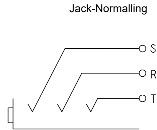
Normalling-Schemes
