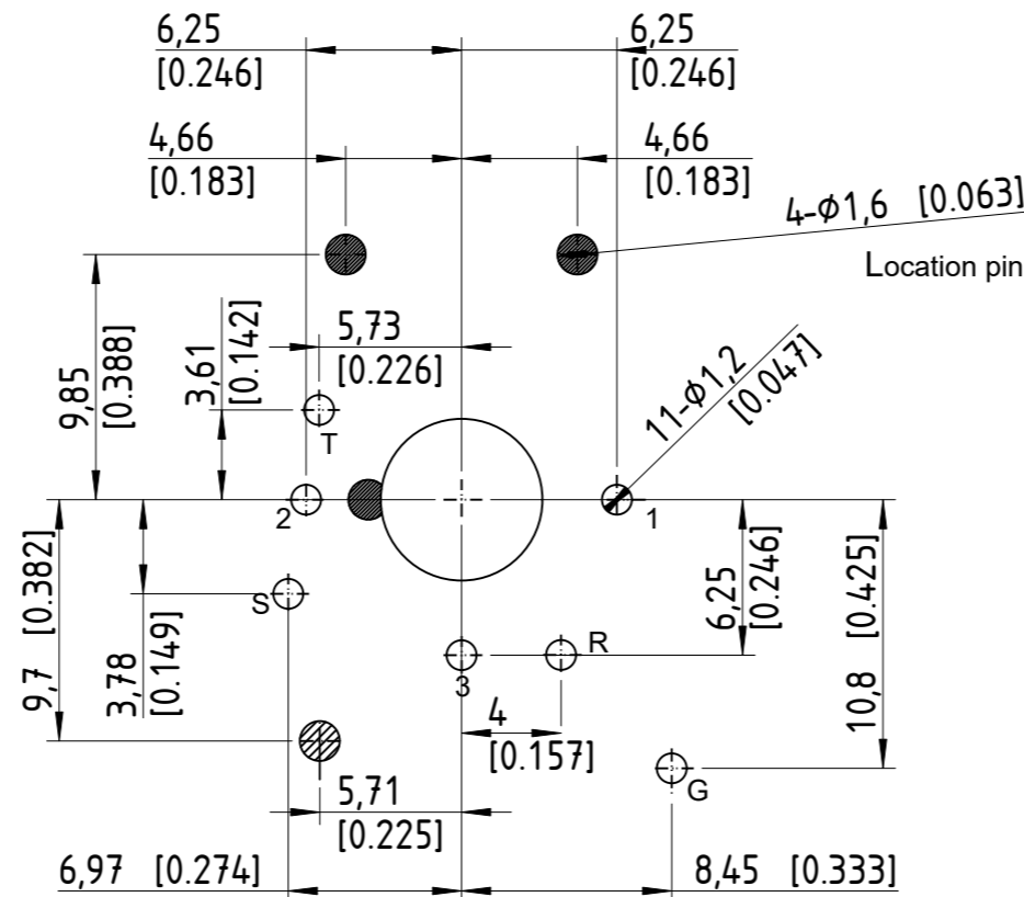
PCB Layout(Component side) tolerance \pm 0.05 [0.002]
